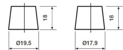
Positive Terminal
